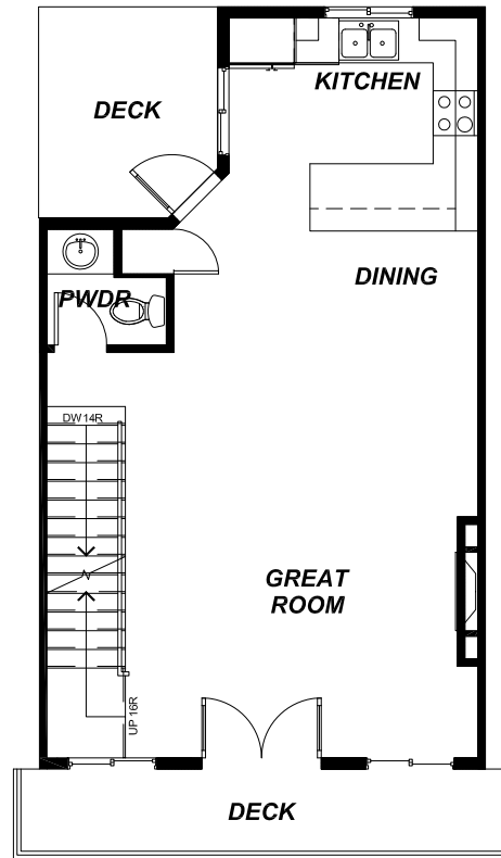
MAIN FLOOR PLAN 605 sf
