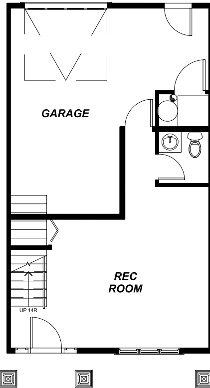
LOWER FLOOR PLAN 364 sf GARAGE 312 sf
