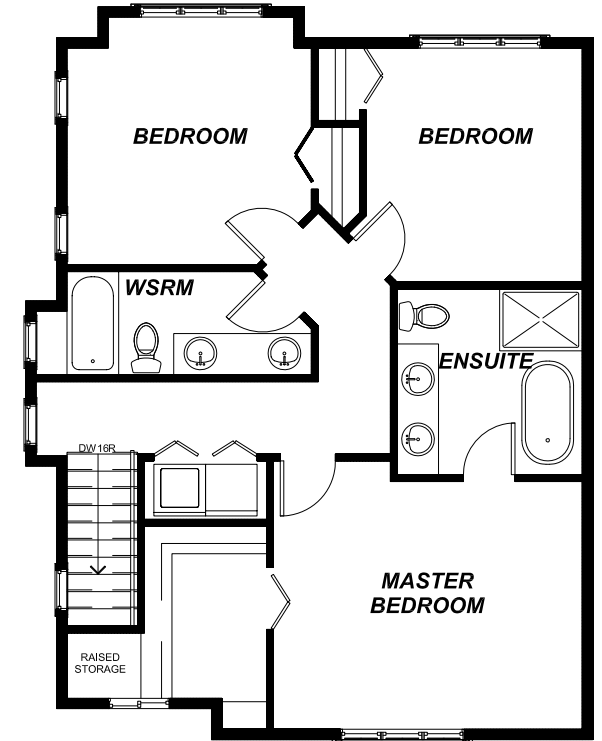
UPPER FLOOR PLAN 900 sf
