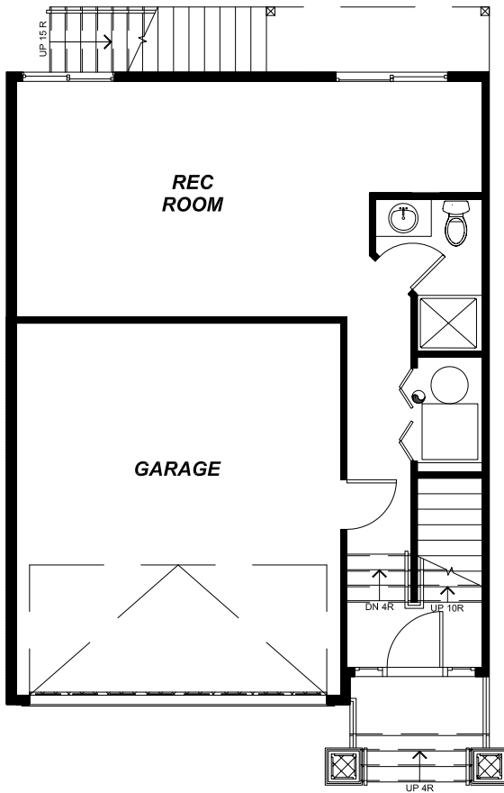
LOWER FLOOR PLAN 491 sf GARAGE 382 sf
