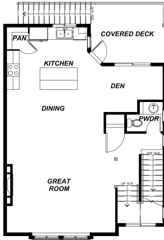
MAIN FLOOR PLAN 800 sf
