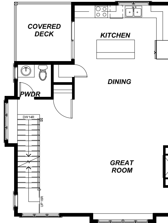
MAIN FLOOR PLAN 765 sf
