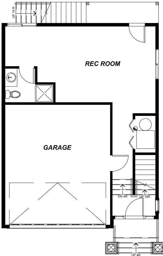
LOWER FLOOR PLAN 490 sf GARAGE 382 sf
