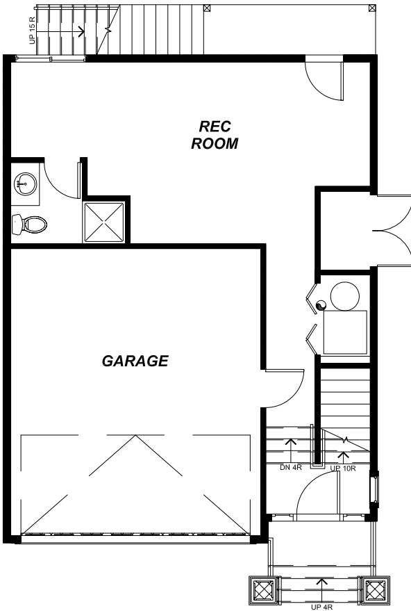
LOWER FLOOR PLAN 495 sf GARAGE 382 sf
