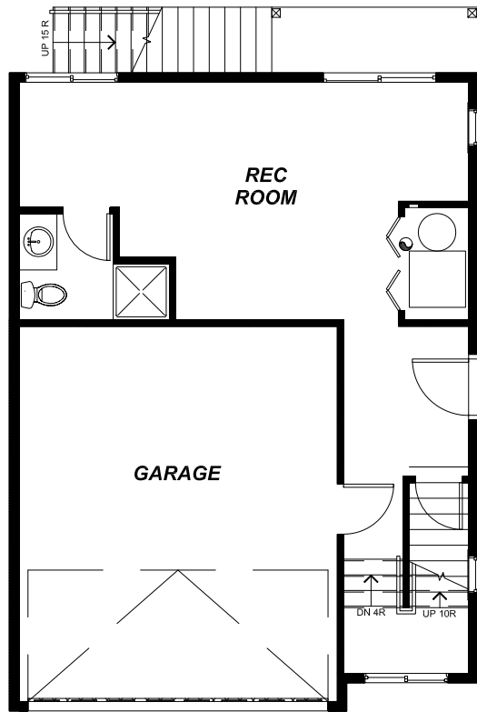
LOWER FLOOR PLAN 468 sf GARAGE 372 sf
