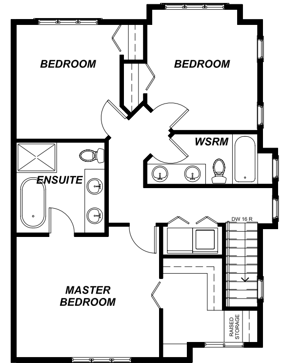
UPPER FLOOR PLAN 866 sf
