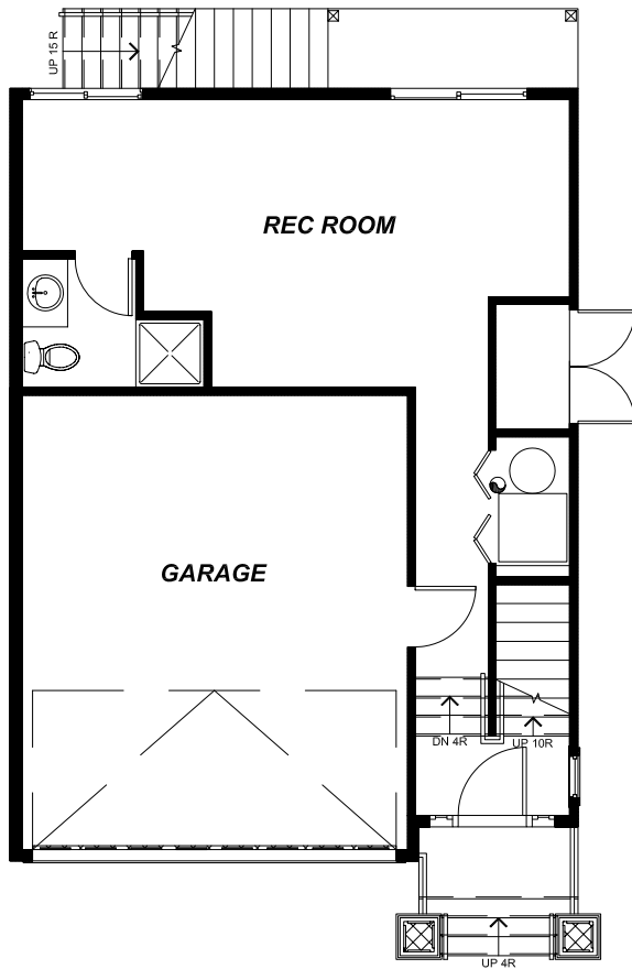
LOWER FLOOR PLAN 443 sf GARAGE 372 sf
