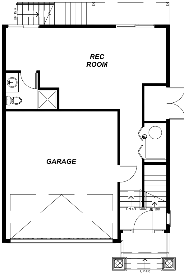
LOWER FLOOR PLAN 491 sf GARAGE 382 sf
