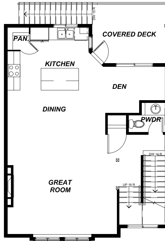
MAIN FLOOR PLAN 800 sf
